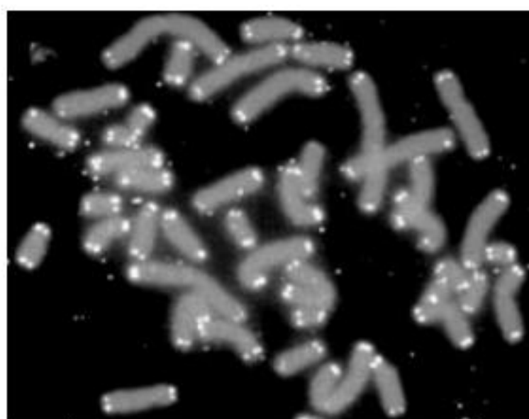
Human chromosomes (grey) capped by telomeres (white)
