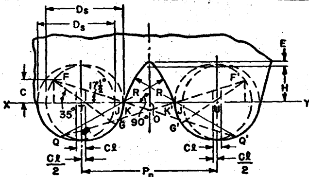
SECTION NORMAL TO HOB TEETH
