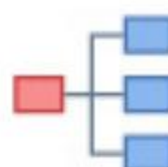
Parallel Tasks
