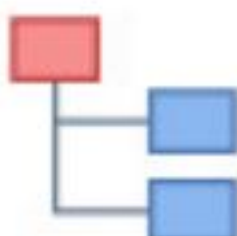
Tree Structure
