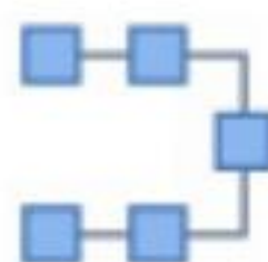
Serial Tasks
