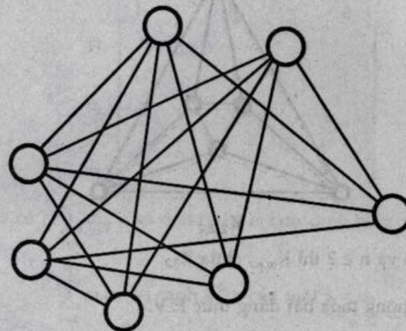
K_{2,2,3}
