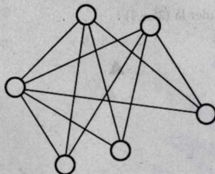
K_{1,2,3}
