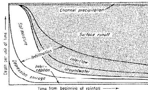
FIGURE 8-3 Schematic diagram of the disposition of storm rainfall.
