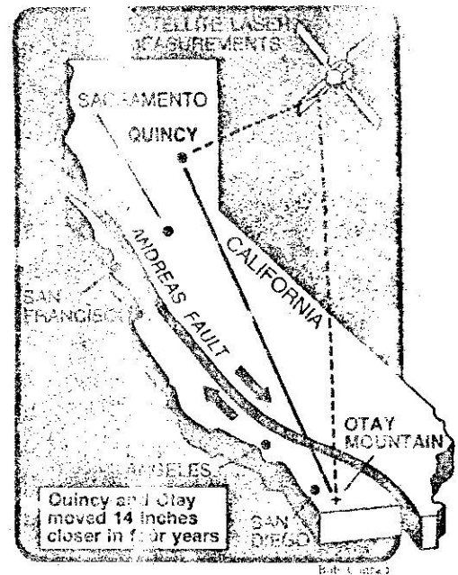
Steady shrinkage: A quake to come?
