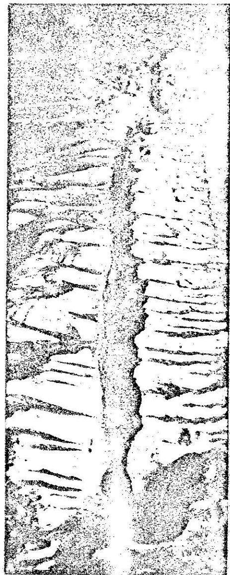
San Andreas Fault Daily grind
