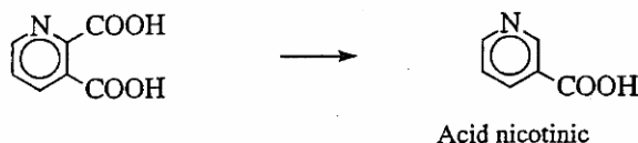
Acid nicotinic
