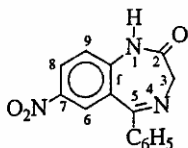
1,3-dihydro-7-nitro 5-phenyl-2H-benzo [f]-1,4-diazepin 2-on (nitrazepam)
