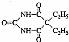
Acid 5,5-diethyl barbituric (Veronal)
