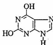
Xanthin (2,6-dihydroxy purin)
