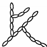
Amylopectin
