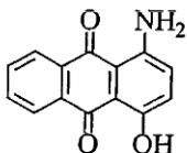
1-Amino-4-hydroxy anthraquinon
