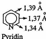
Pyridin
