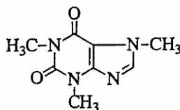
Cafein
