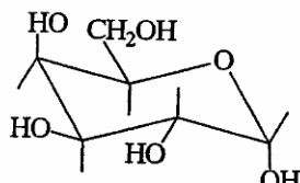
\alpha -D-galactopyranose
