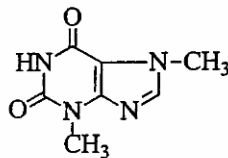
Theobromin
