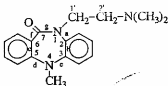
1-(2'-dimethylaminoethyl)-4-methyl-7-oxo dibenzo [b,e] 1,4-diazepin
