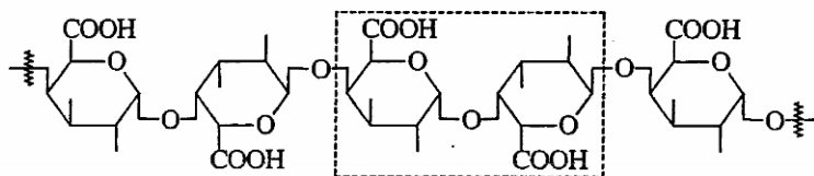
Acid D-galacturonic
