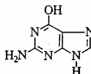
Guanin (2-amino 6-hydroxy purin)
