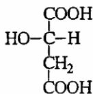
acid L(-) malic
