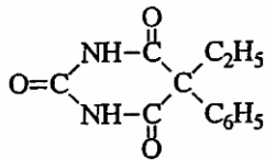
Acid 5-ethyl-5-phenyl barbituric (Luminal)
