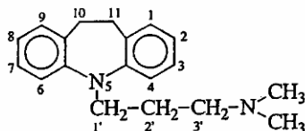
5-(3'-dimethylaminopropyl)-10,11-dihydro-5H-dibenzo [b,f] azepin (imipramin : chống trầm uất)
