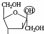
\beta -D-fructofuranose
