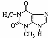
Theophyllin
