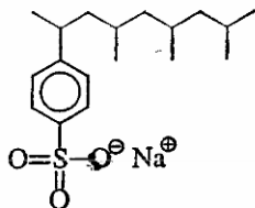
Natri alkyl benzensulfonat
