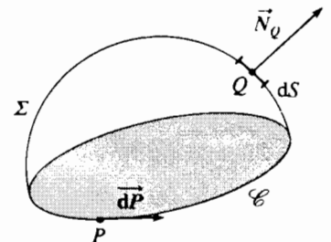
H.55. Định lý STOKES-AMPÈRE \oint_{\mathcal{C}} \vec{G}(P) \cdot d\vec{P} = \iint_{\Sigma} \text{rot}(\vec{G}(Q)) \cdot \vec{N}_Q dS.
